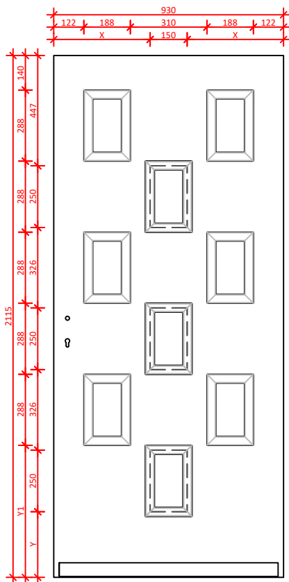
Laag model 1900 - 2200
