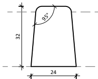
Verticale lat
