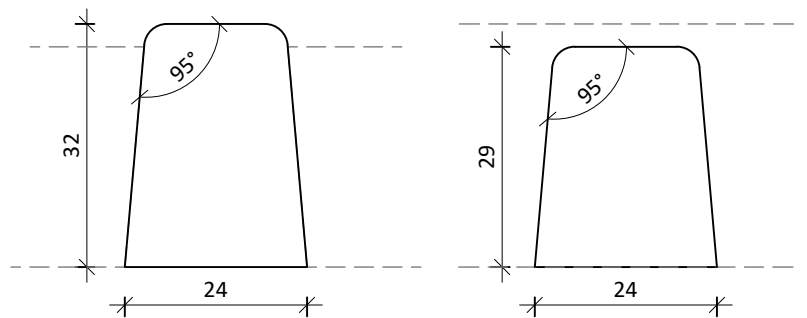
Verticale lat
