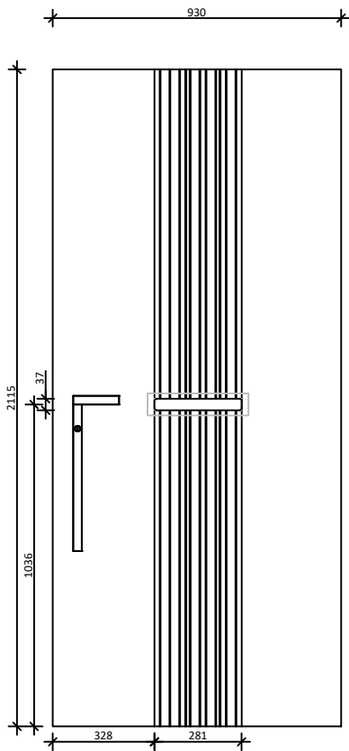
Laag model 1900 - 2200
